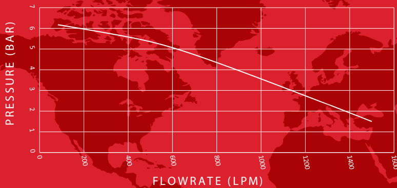
P1 GASOLINE MOTOPUMP PERFORMANCE CURVE
